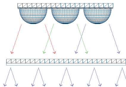
Light Ray Diagram
