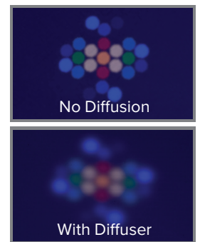
Pinhole Projection Image
